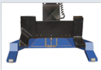
Universal lifting carriages with two flat, sliding support forks to hold forklift trucks etc.
